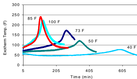
Typical Exotherm Curve for MA590 in a 100 gm Mass at Various Ambient Temperatures at 74°F 5
