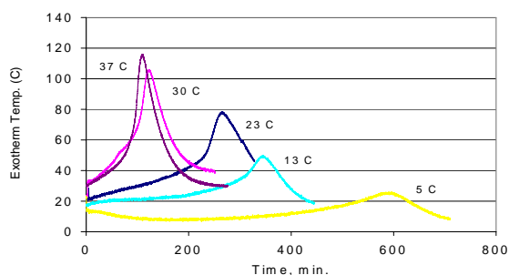
Typical Exotherm Curve for MA590 in a 100 gm Mass at Various Ambient Temperatures at 74°F 5
